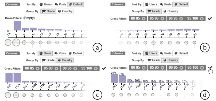
Fig. 4. An example of using crossing filtering in the Matrix View. (a) Users are grouped by grade in the matrix diagram. (b) Analysts create filters by clicking the column labels. (c) Users are grouped by country. (d) Analysts apply the filters by clicking the “✓” on the toolbar. The top five countries with the highest achieving students are revealed: India, the USA, Spain, Great Britain, and Canada.
